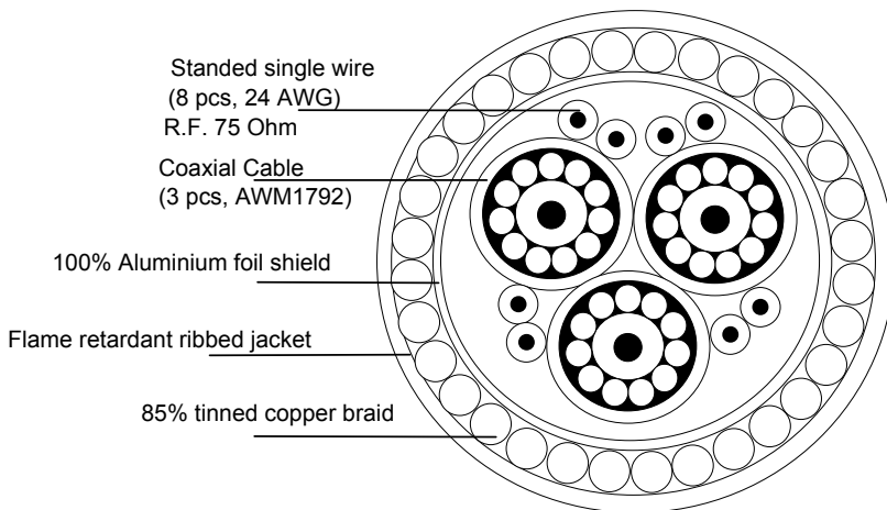
RGB CABLE Not to scale
